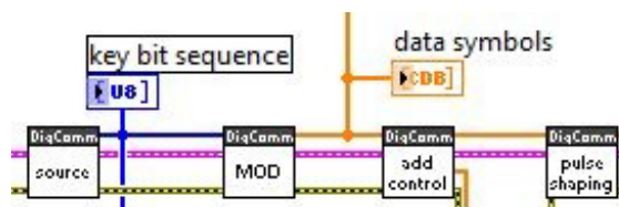
Figure 4: Block diagram of transmitter.vi .
