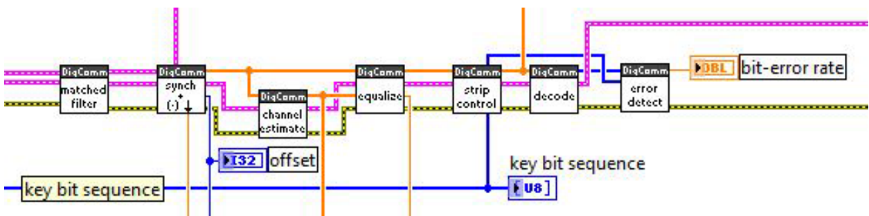
Figure 6: Block diagram of receiver.vi .
